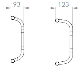
HUM030403 & HUM030404 Stabilizer bar close & wide
